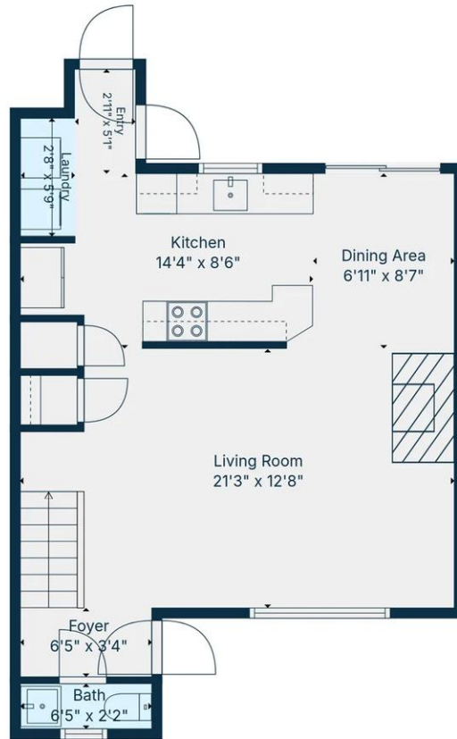
1st Floor
